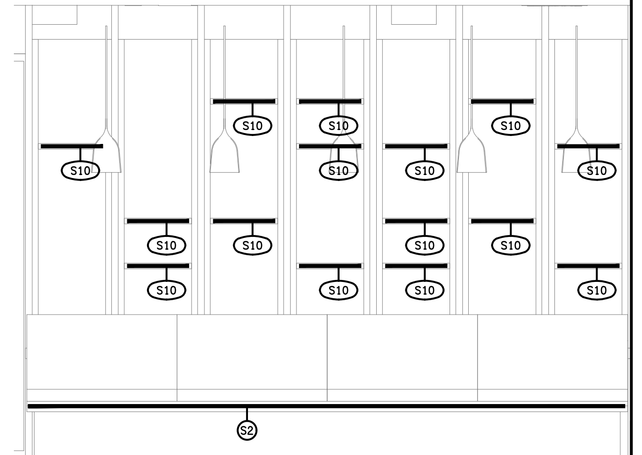
DETAIL D BISTRO DINING FEATURE WALL ELEVATION SCALE 1: 25
